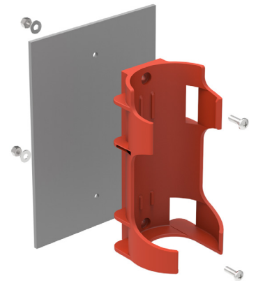
Bracket Mounting Option
